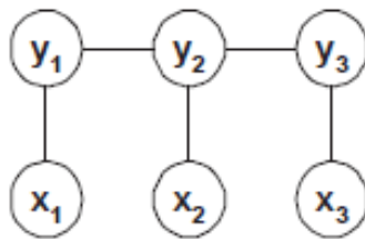
FIGURE 5: Graphical model representation of and chain-structured CRF
