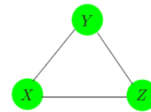
FIGURE 3. A complete graph does not uniquely specify the higher-order dependence structure in the joint distribution of the variable.
